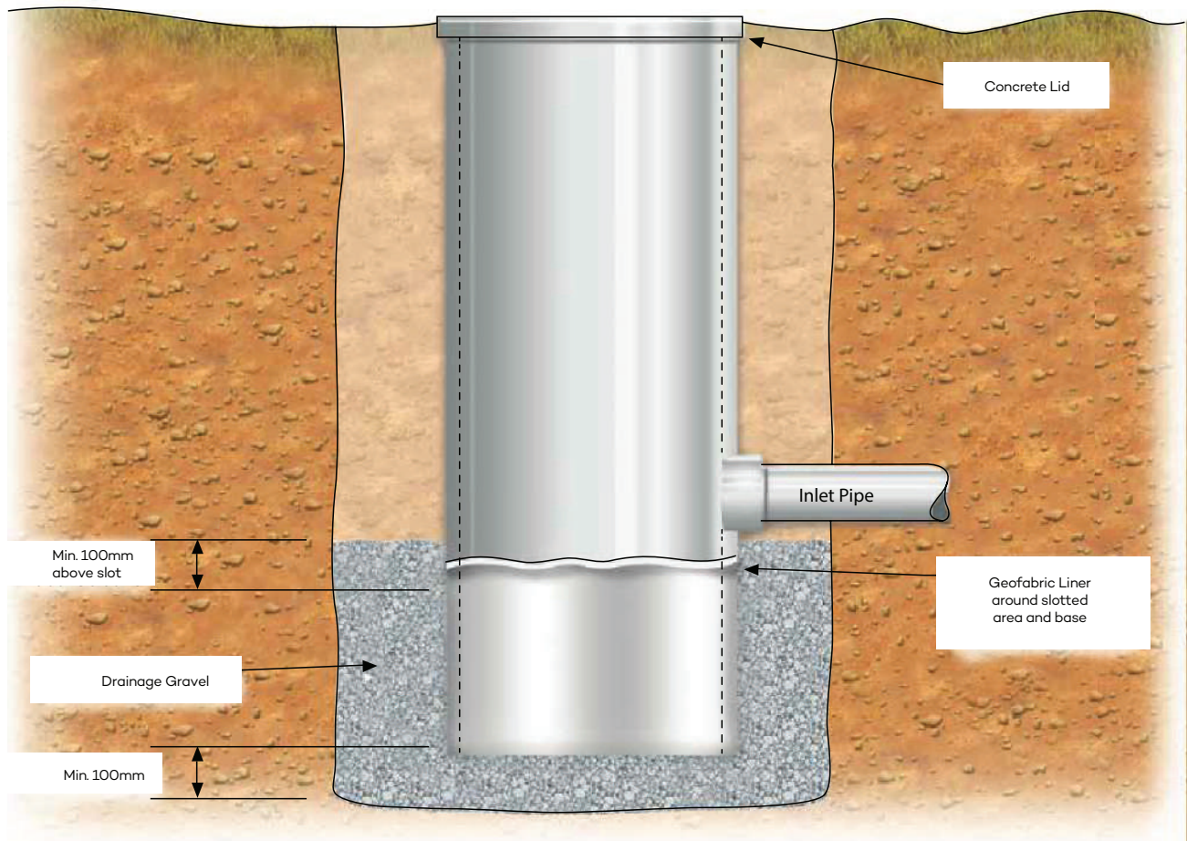
FRC AQUIFER Soakwell Pit
