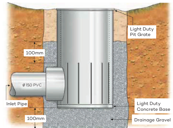
FRC AQUIFER Surcharge Pit
