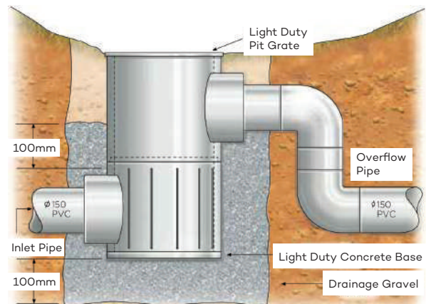
FRC AQUIFER Discharge Pit
